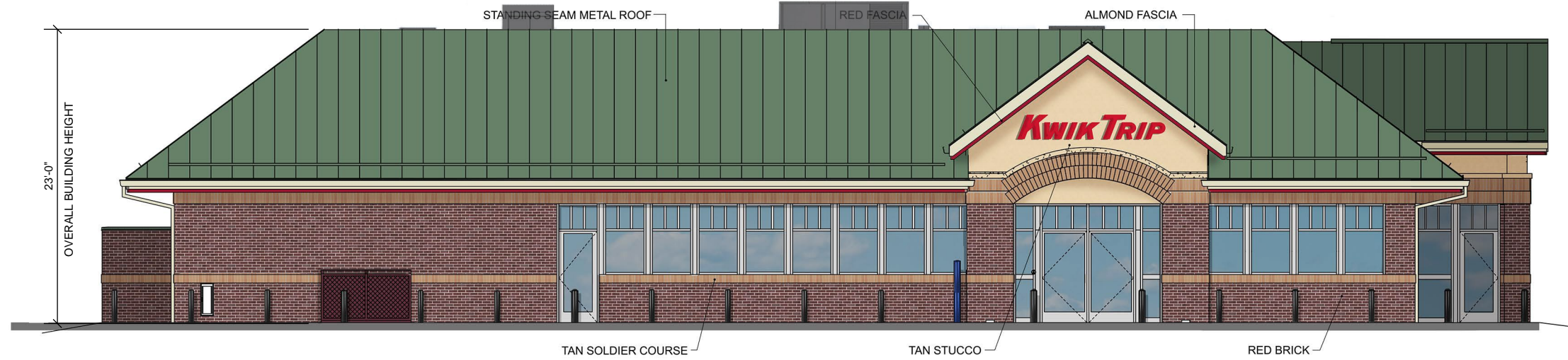
1 FRONT ELEVATION
