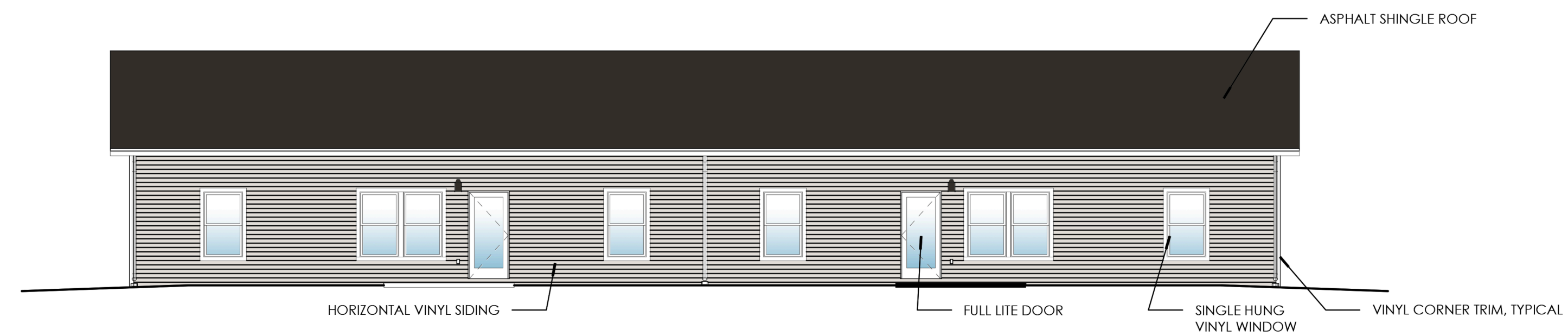
4 REAR ELEVATION 1/8" = 1'-0"
