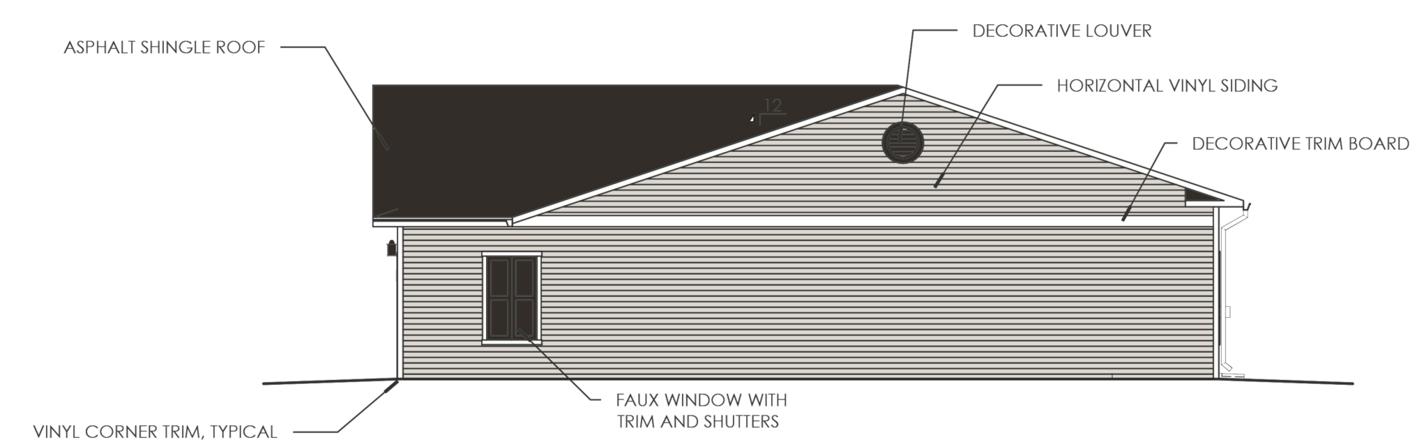
3 SIDE ELEVATION 1/8" = 1'-0"
