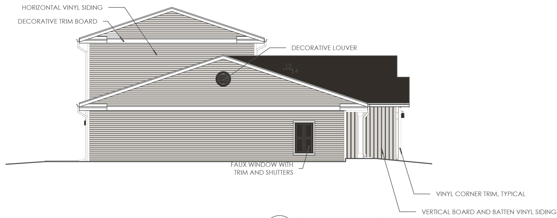
2 SIDE ELEVATION 1/8" = 1'-0"
