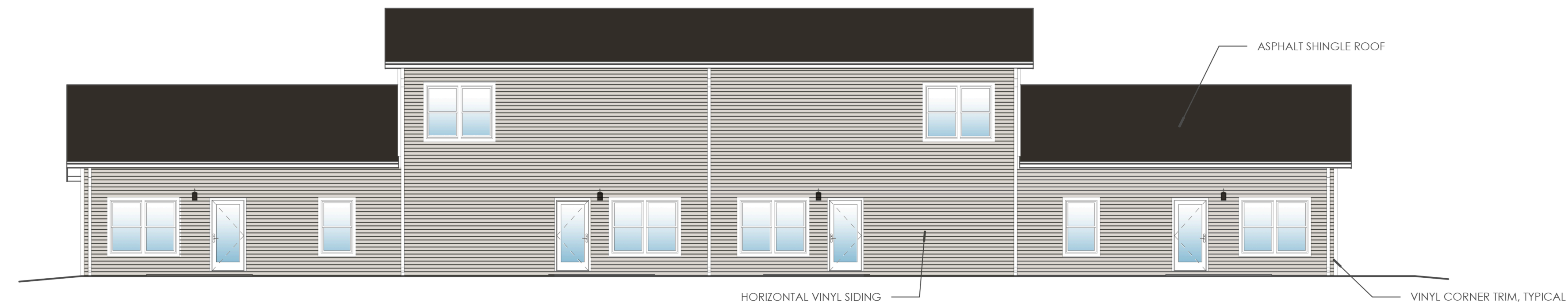
4 REAR ELEVATION 1/8" = 1'-0"
