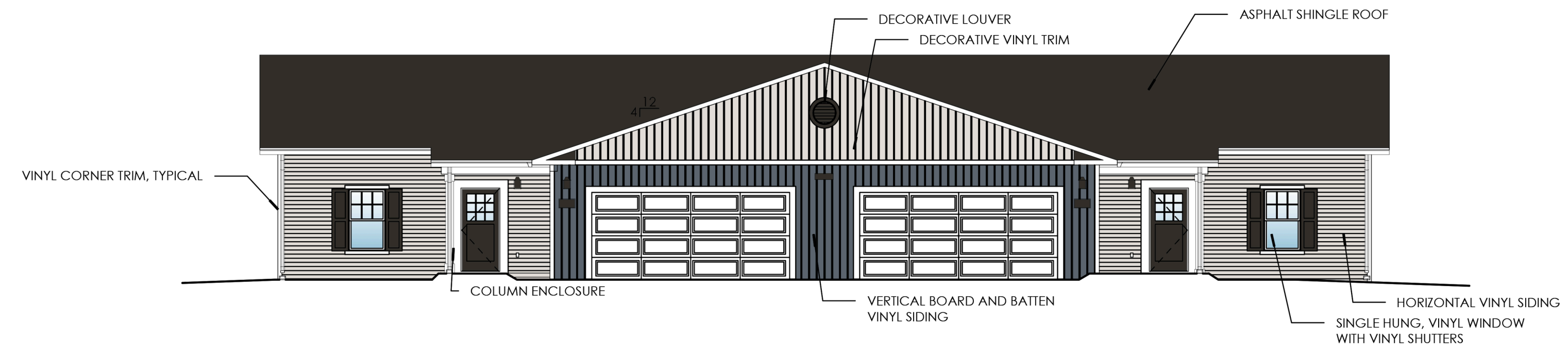
1 FRONT ELEVATION 1/8" = 1'-0"
