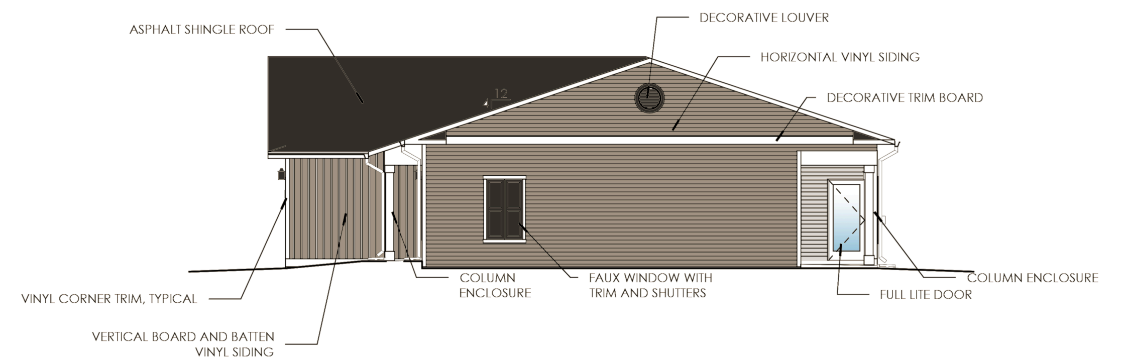
3 SIDE ELEVATION 1/8" = 1'-0"
