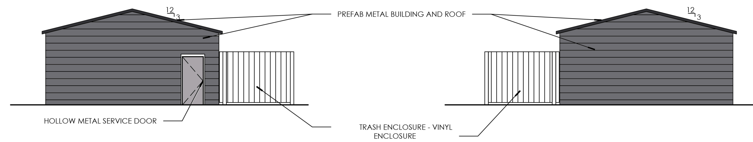
2 SIDE ELEVATION 1/8" = 1'-0"
