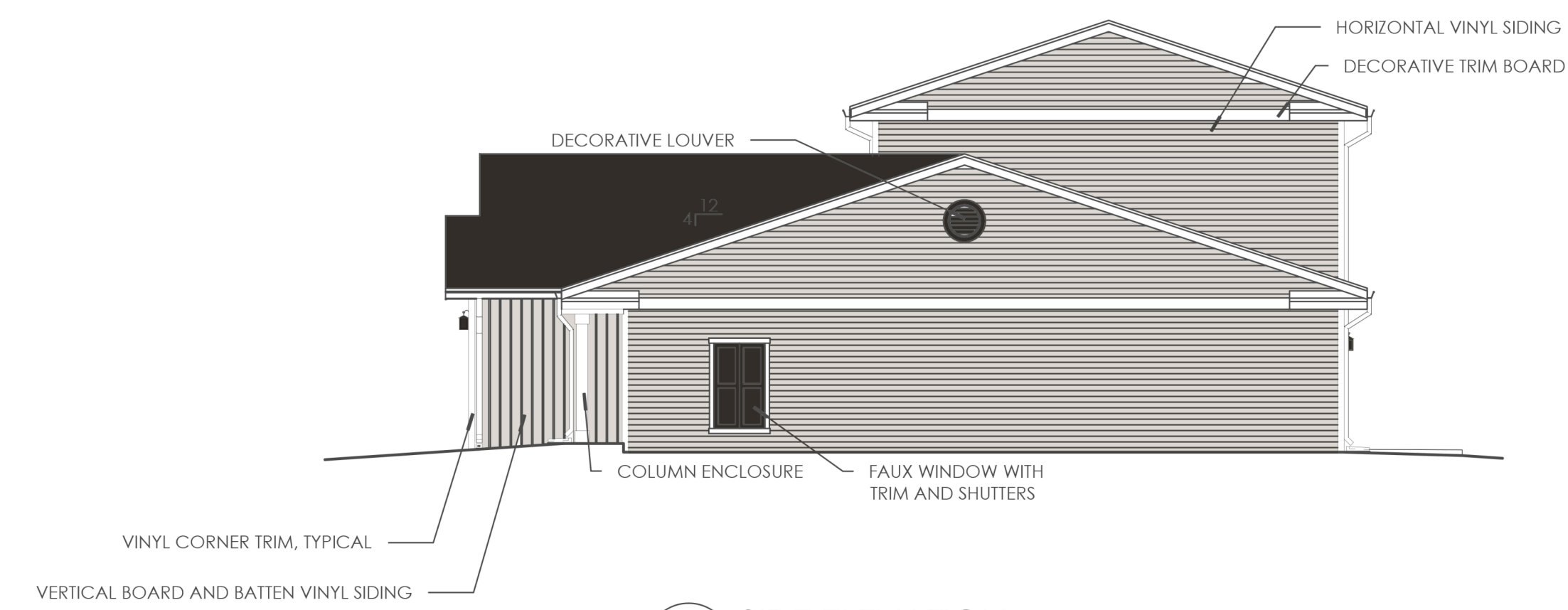
3 SIDE ELEVATION 1/8" = 1'-0"
