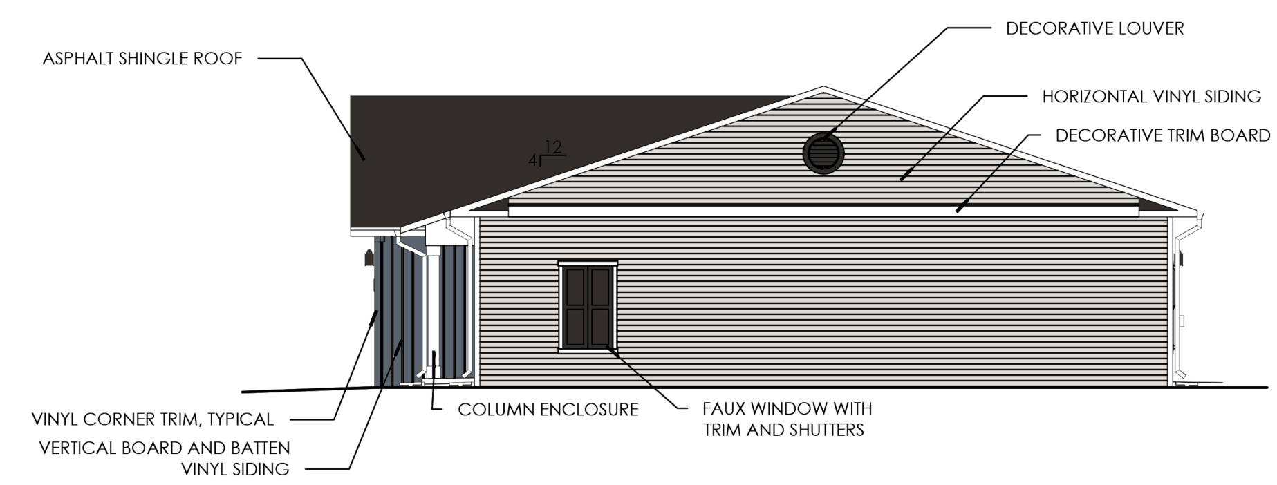
3 SIDE ELEVATION 1/8" = 1'-0"
