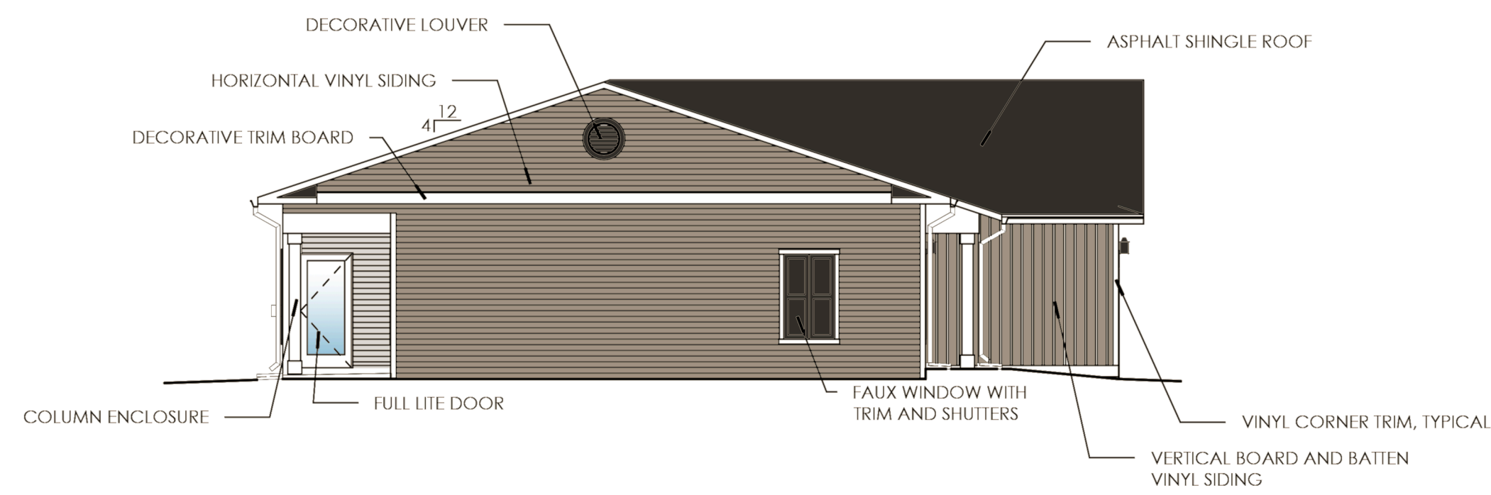
2 SIDE ELEVATION 1/8" = 1'-0"
