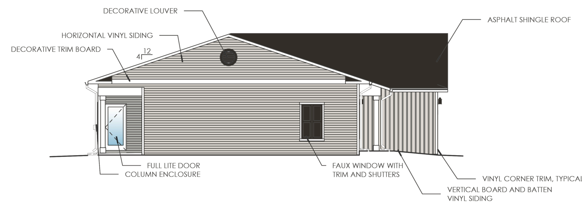
2 SIDE ELEVATION 1/8" = 1'-0"
