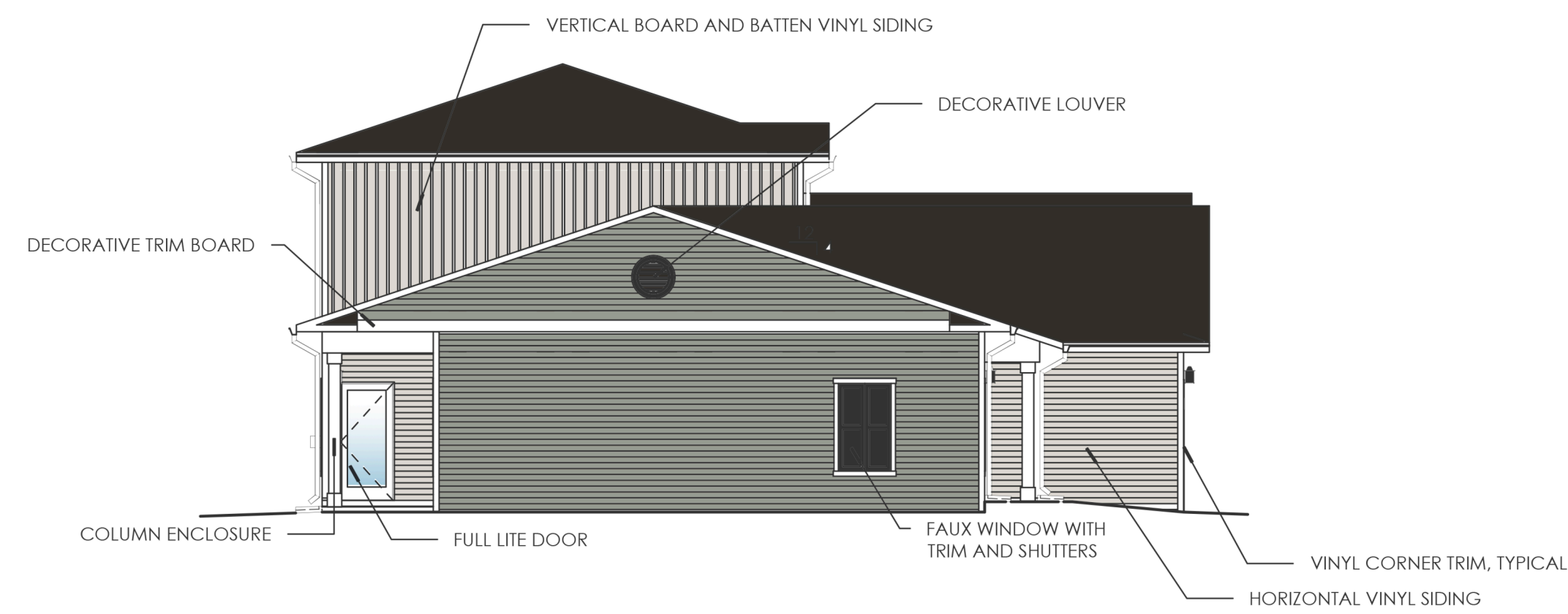
2 SIDE ELEVATION 1/8" = 1'-0"
