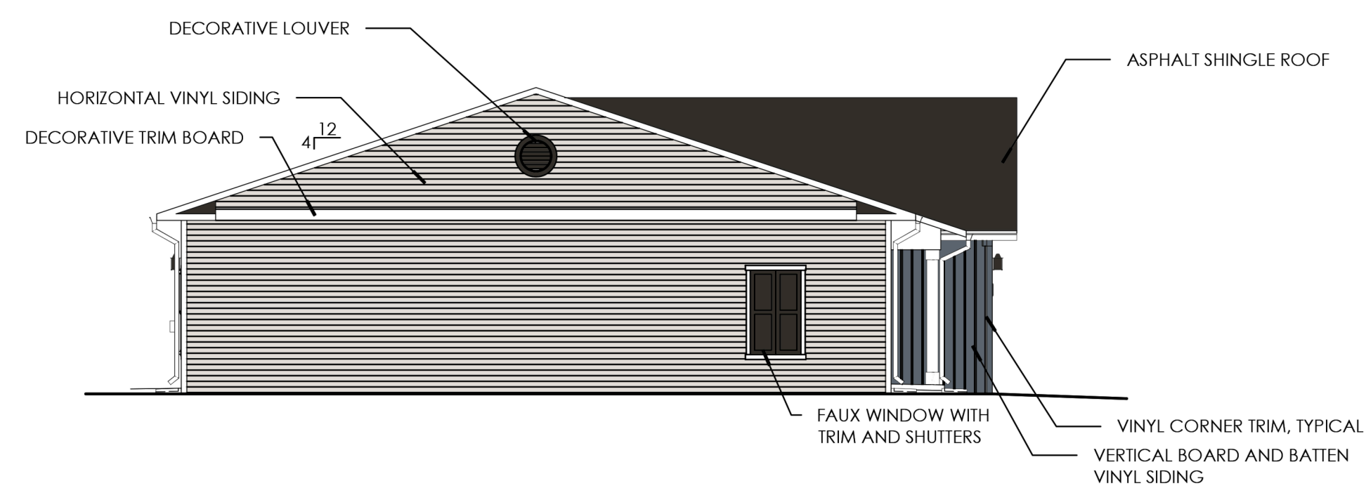
2 SIDE ELEVATION 1/8" = 1'-0"
