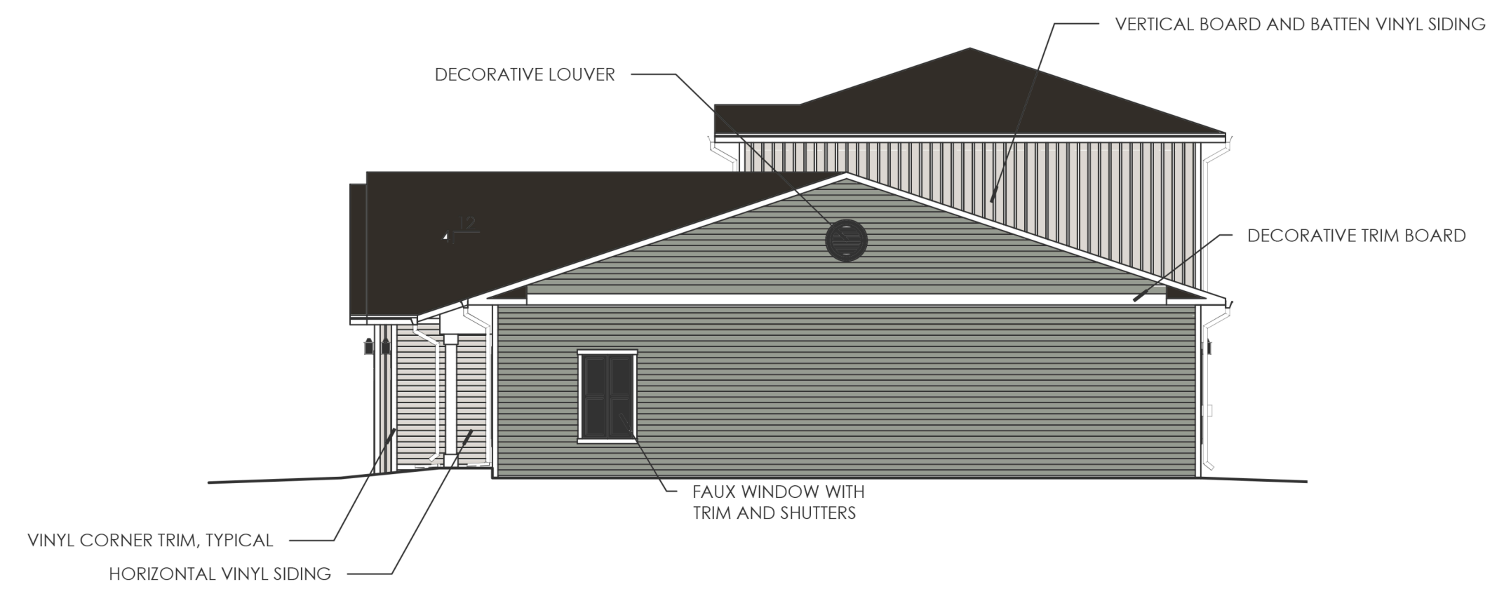
3 SIDE ELEVATION 1/8" = 1'-0"
