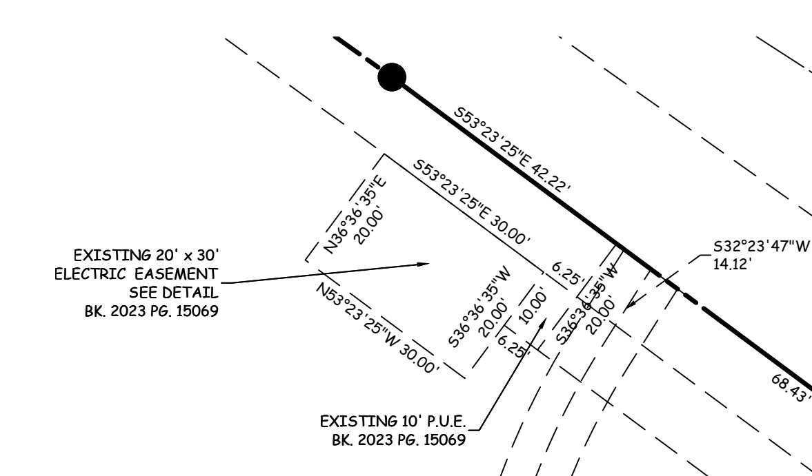
EASEMENT DETAIL SCALE: 1"=20'
